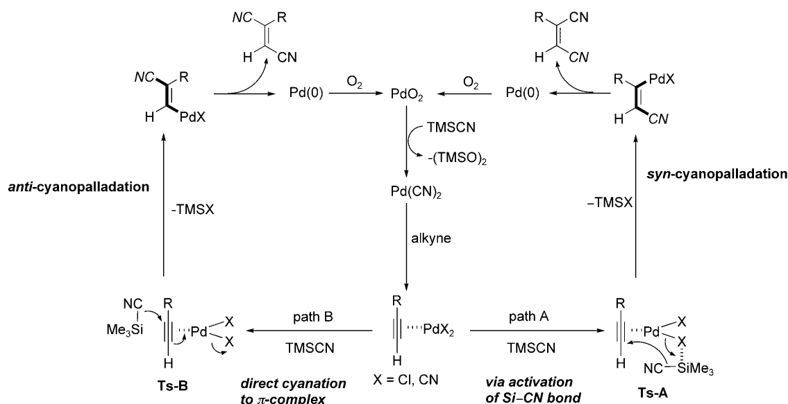
Scheme 2. Plausible catalytic cycle for the 1,2-dicyanation of terminal alkynes.
