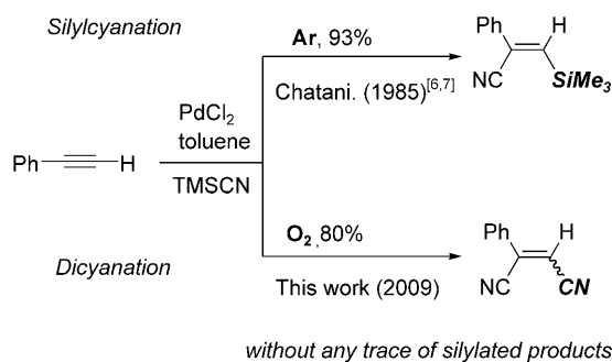
Scheme 1. Pd-catalyzed cyanation of phenylacetylene with TMSCN.
