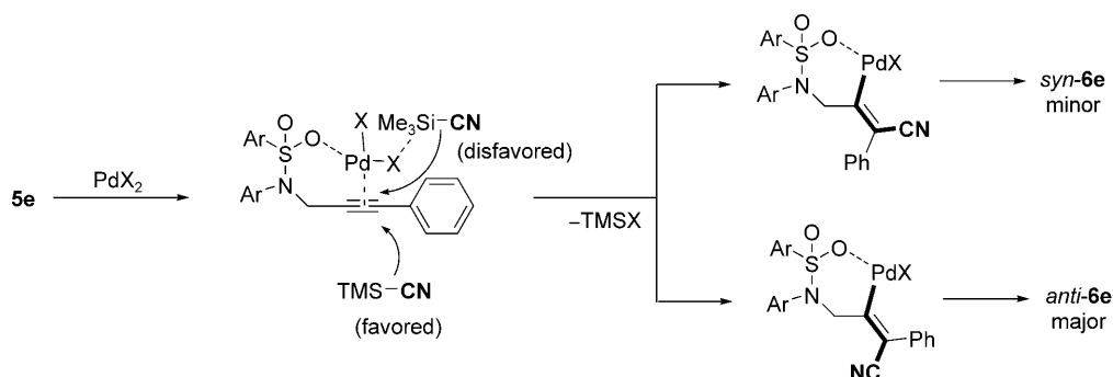
Scheme 3. Plausible reaction pathways from 5e .
