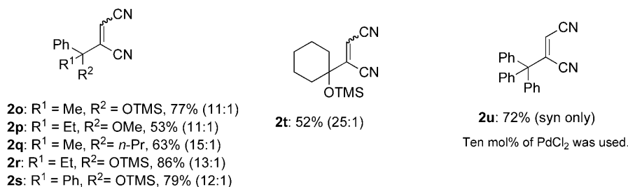
Figure 1. Products, yields and syn/anti ratios in the 1,2-dicyanation of terminal alkynes bearing a tetrasubstituted carbon at the propargyl position.
